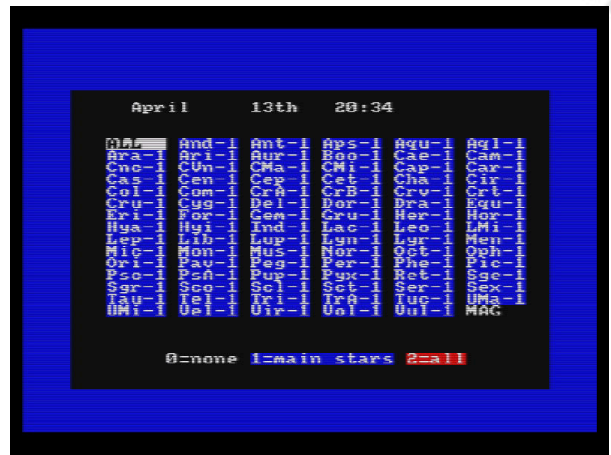
Figure 13 - Magnitude selection
