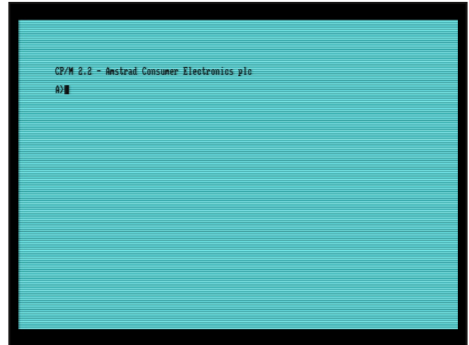
Figure 2 - CP/M 2.2
