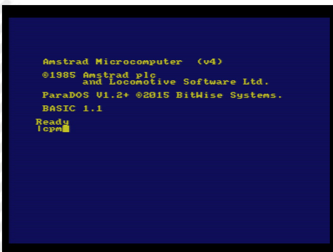
Figure 1 - Command |cpm
